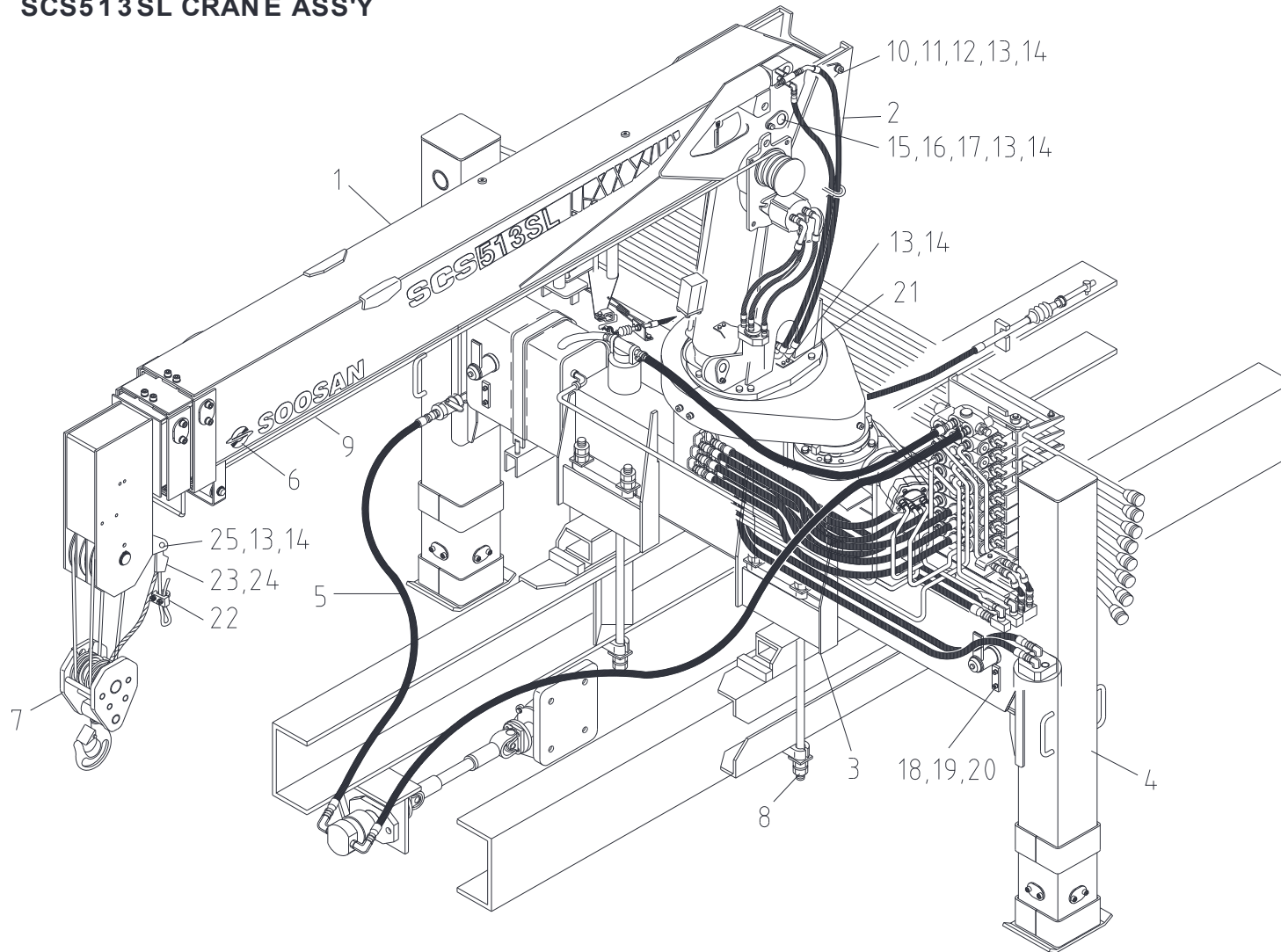
Fig. 0 SCS513SL CRANE ASS'Y
