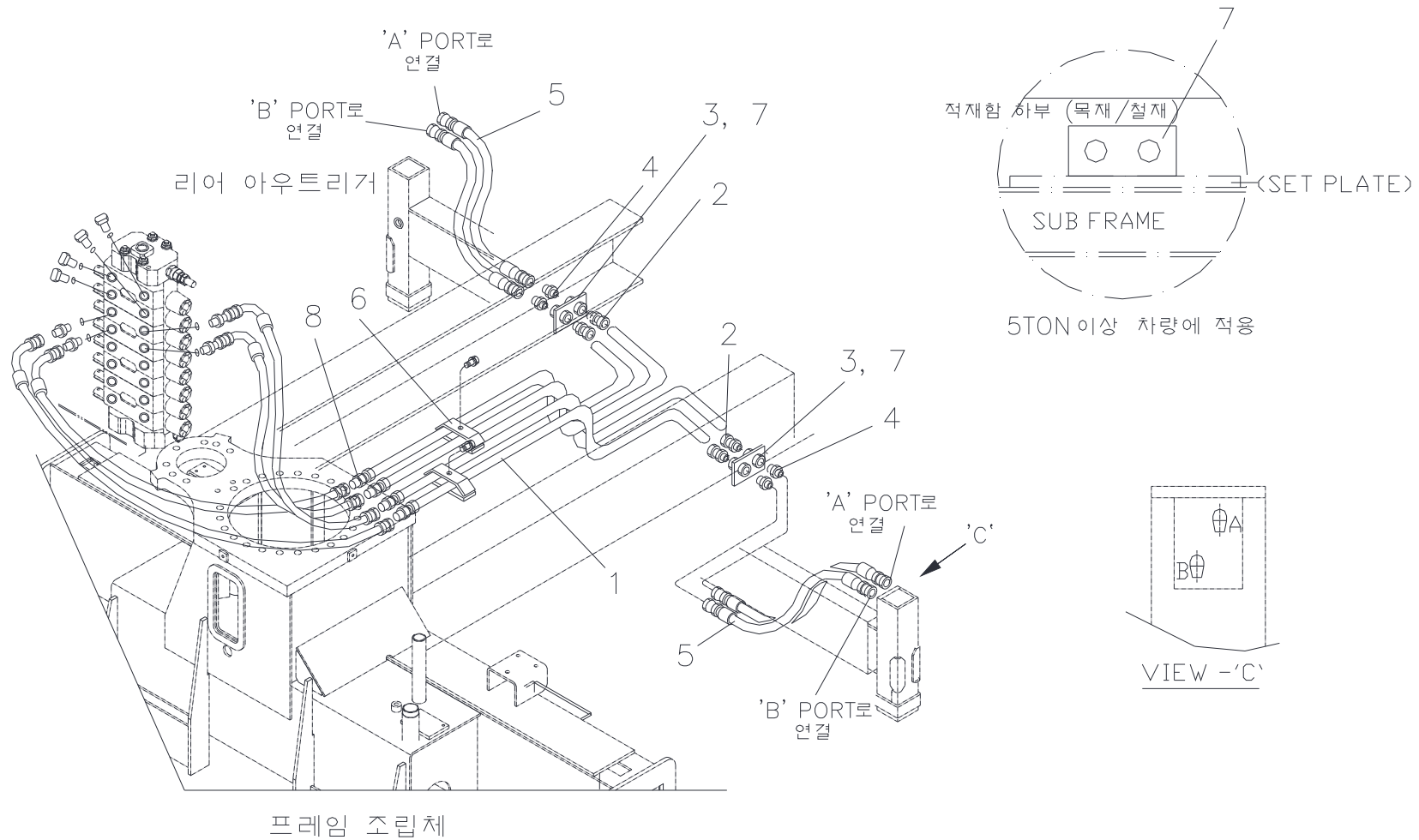
Fig. 8-4 SCS513SL R/ O M/ T PIPING PART
