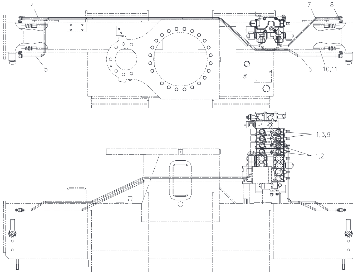
Fig. 5-6 SCS513SL OUTRIGGER PIPING
