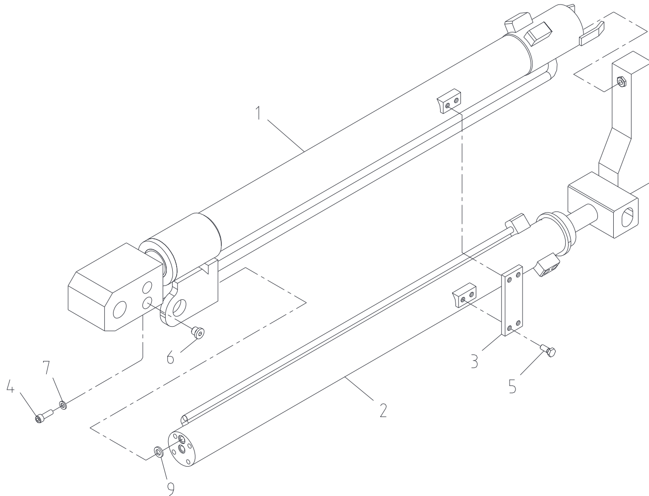
Fig. 1-1 SCS513SL TELESCOPIC CYL' ASS'Y
