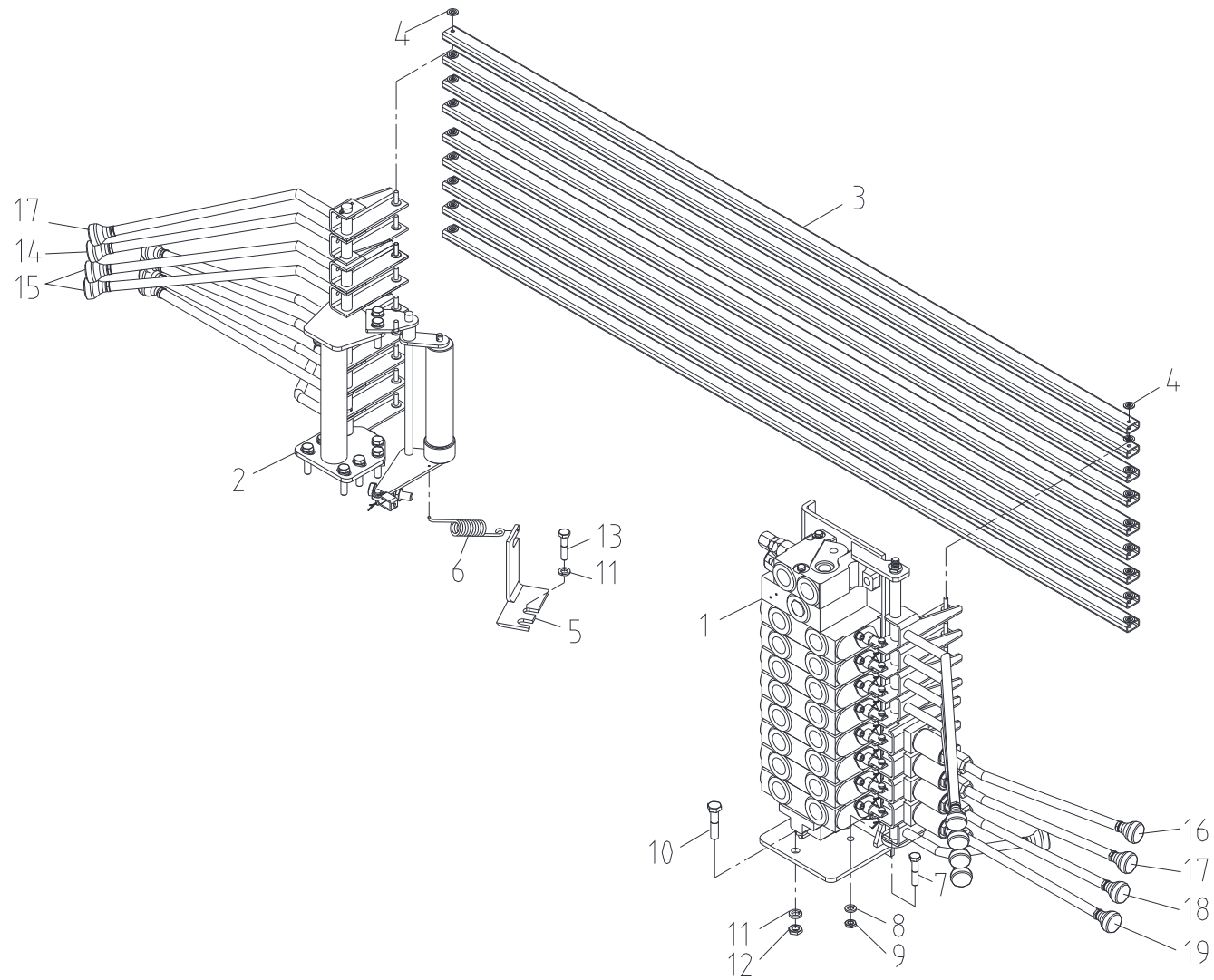
Fig. 3-4 SCS513SL OPERATION MAIN ASS'Y
