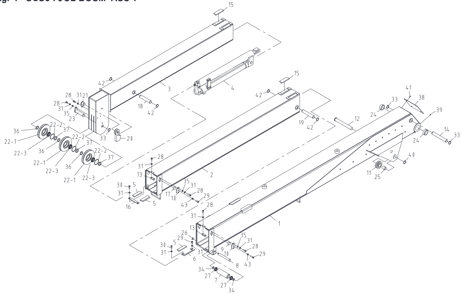
Fig. 1 SCS513SL BOOM ASS'Y
