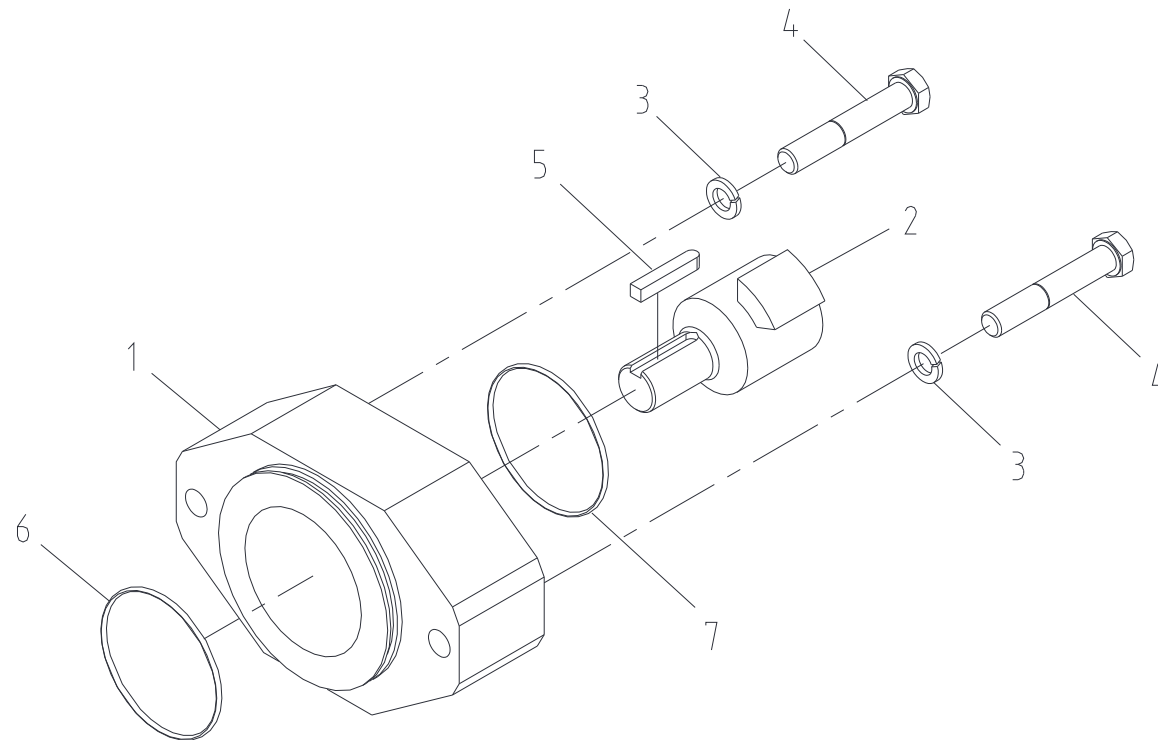
Fig. 3-2 SCS513SL SWING R/G ADAPTER ASS'Y
