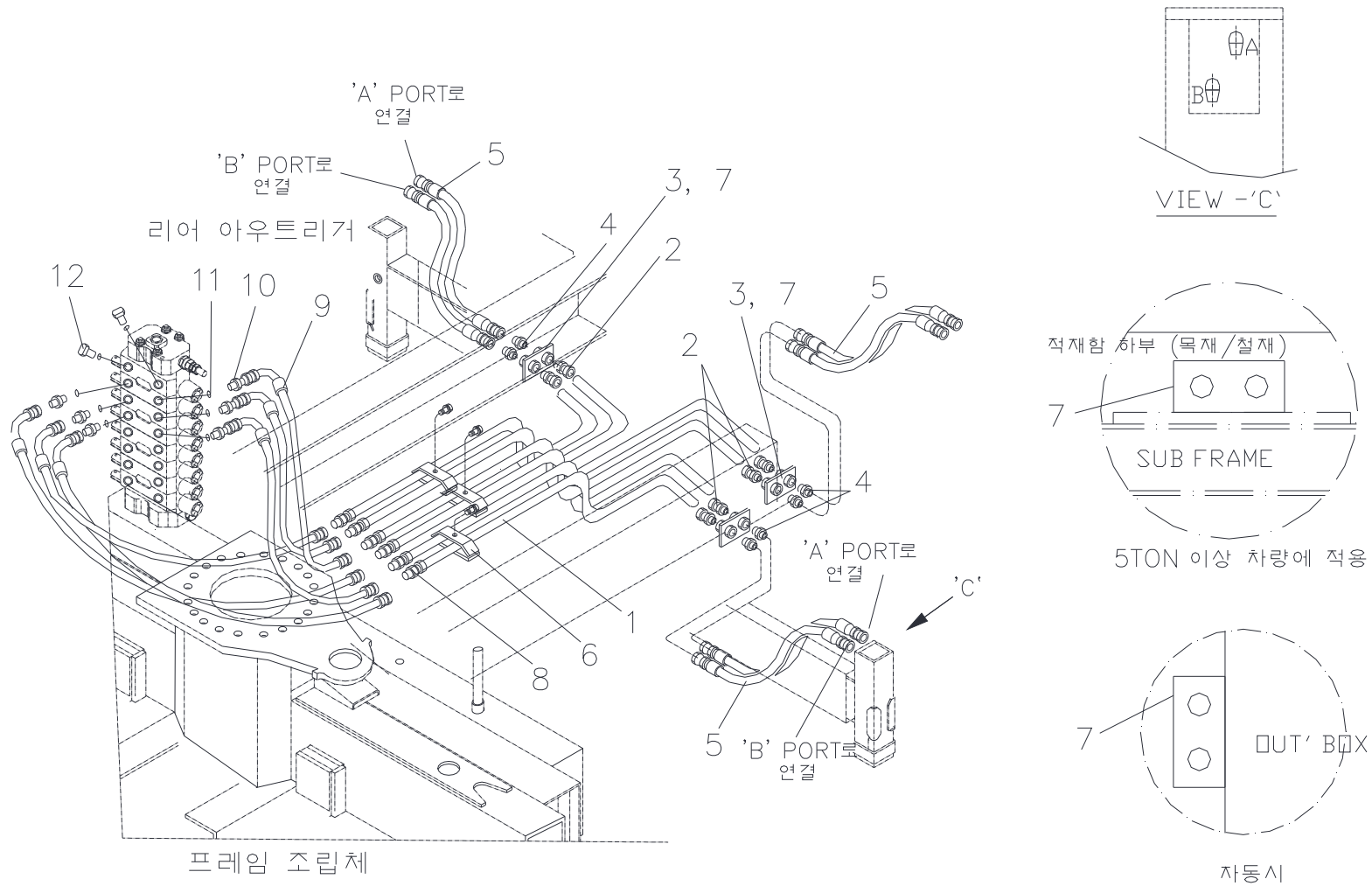
Fig. 8-4 SCS513SL R/ A M/ T PIPING PART
